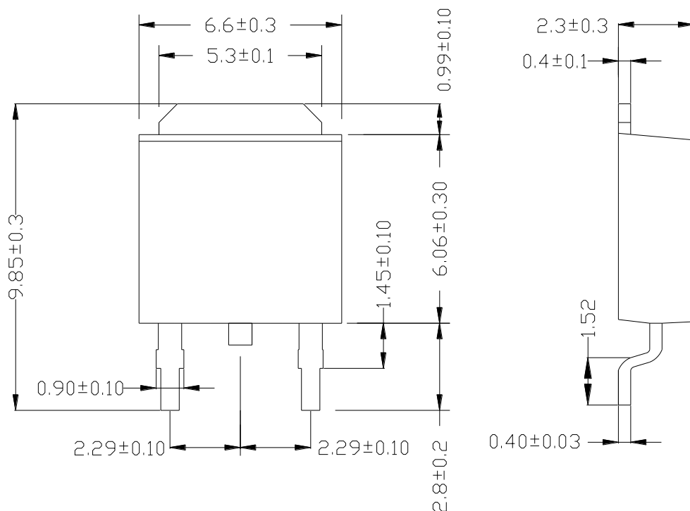
T0-252
