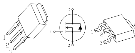
TO-251S
