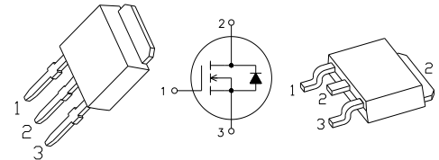
TO-251S
