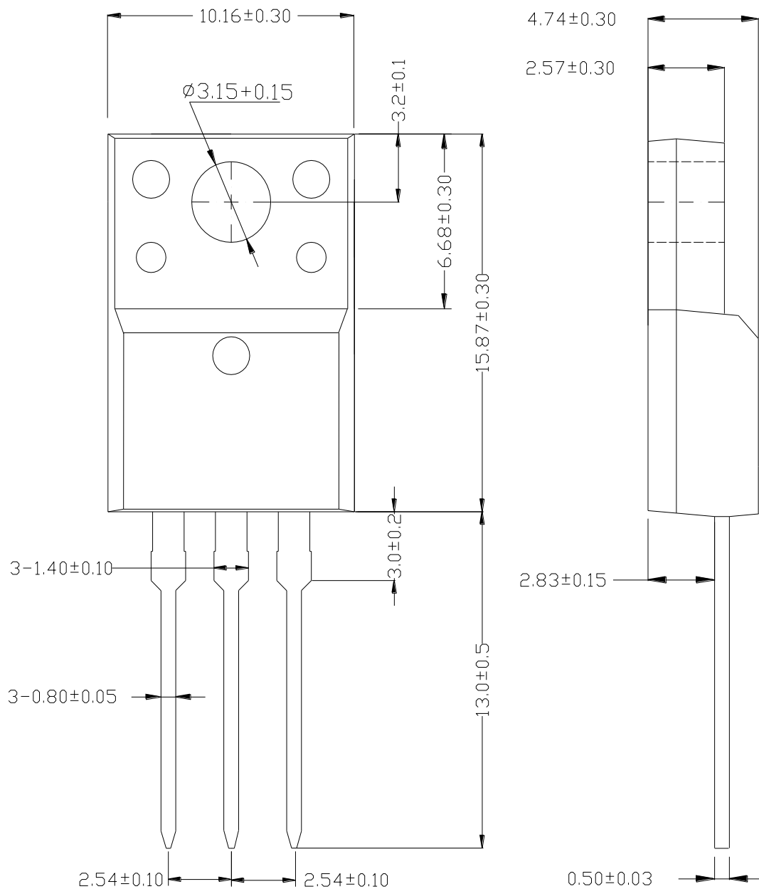
TO-220F
