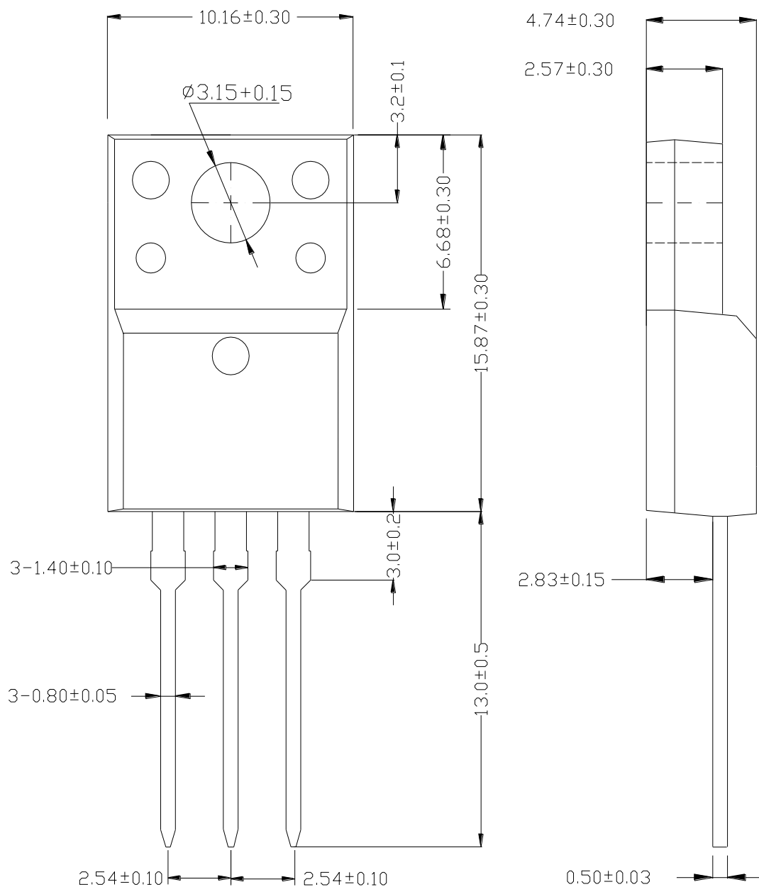
T0-220F
