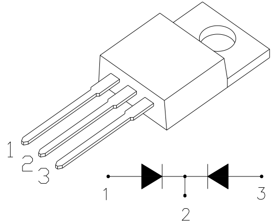
1. 阳极(A1) 2. 阴极(K) 3. 阳极(A2)
