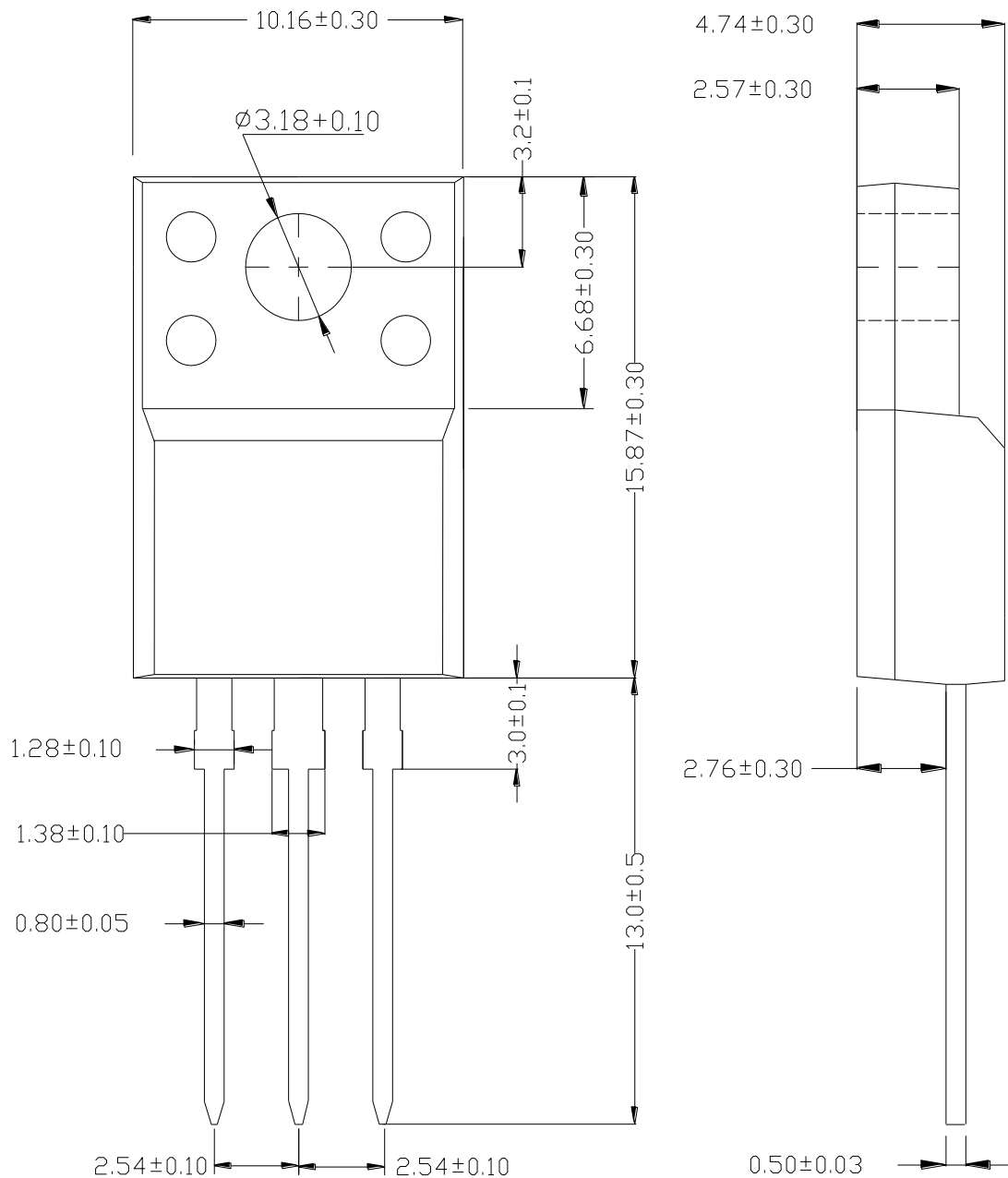
T0-220F
