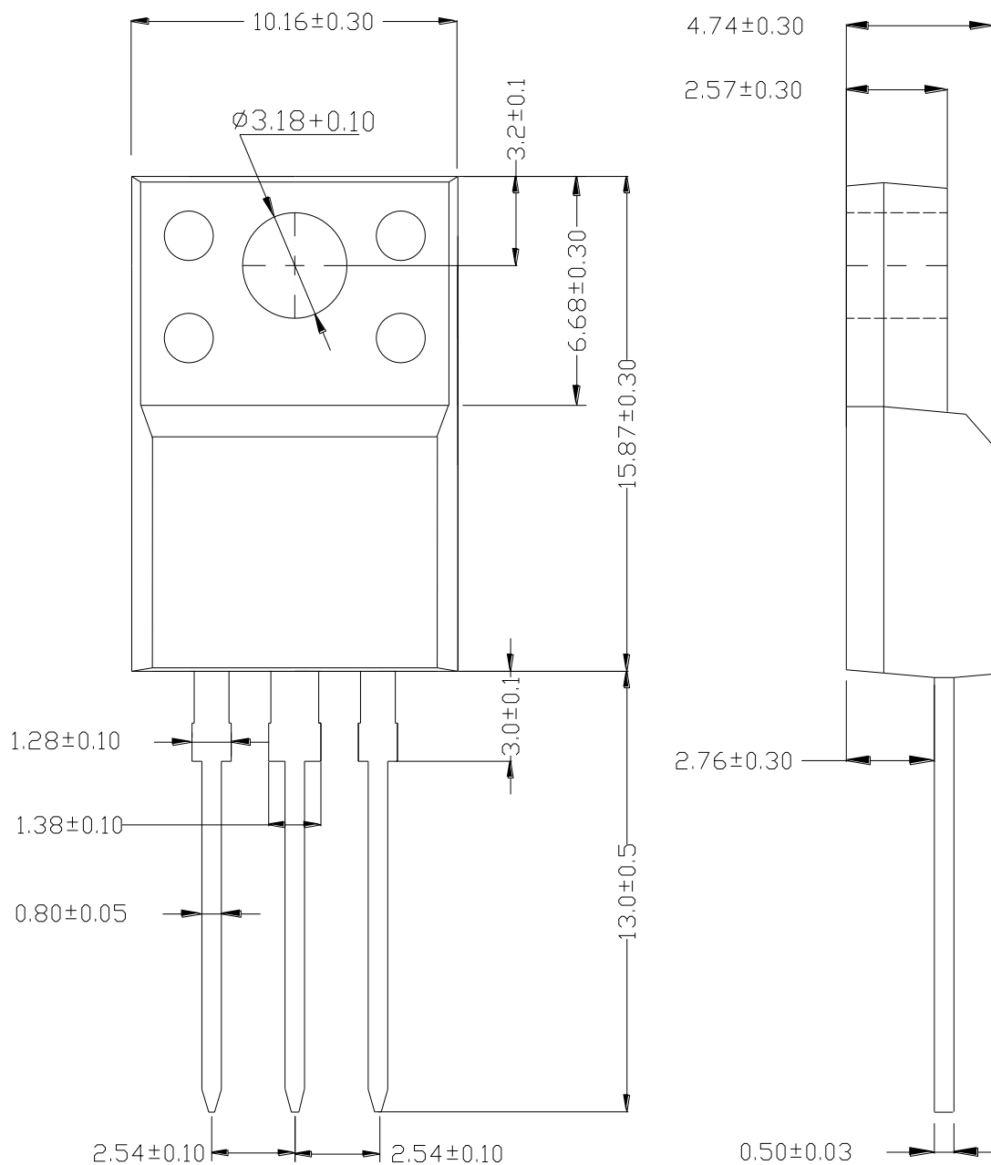
T0-220F
