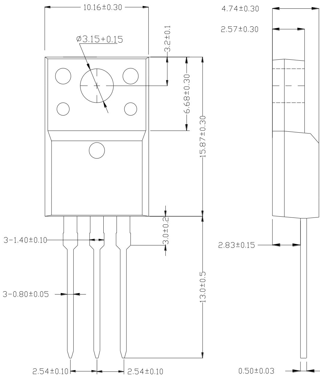
T0-220F
