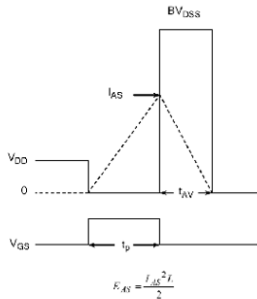
Figure 24. Undamped Inductive Switching Waveforms
