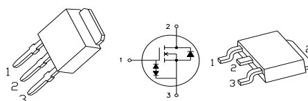
TO-251S
