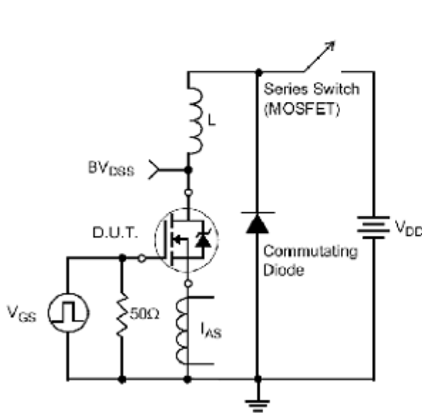
Figure 23. Undamped Inductive Switching Test Circuit
