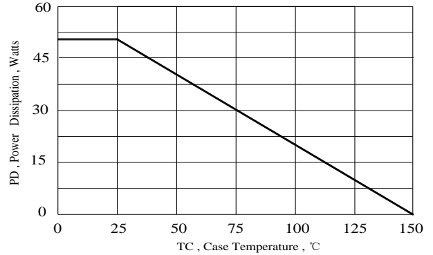
Figure 2, Maximum Power Dissipation vs Case Temperature
