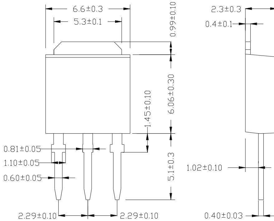
T0-252S
