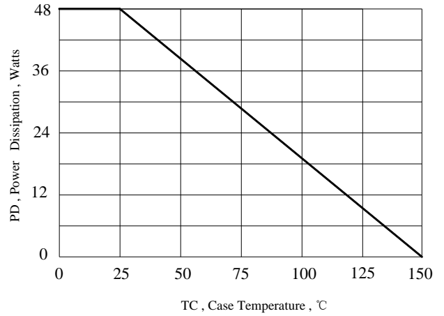
Figure 2 Power Dissipation vs Case Temperature
