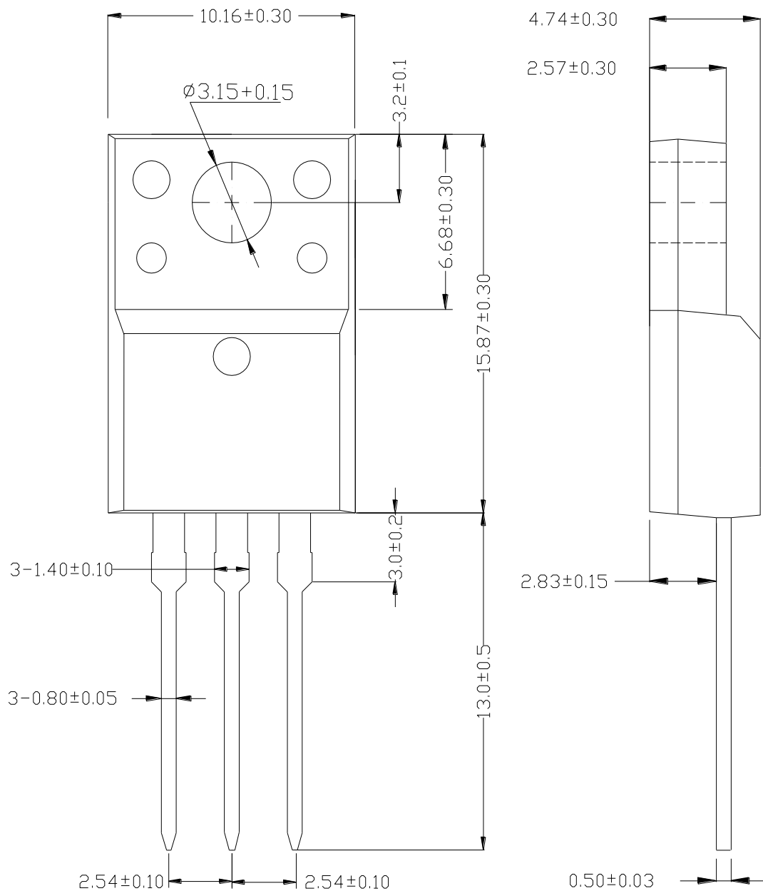
TO-220F
