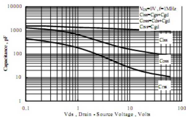
Figure 13 Typical Capacitance vs Drain to Source Voltage
