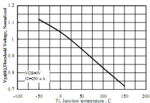
Figure 11 Typical Threshold Voltage vs Junction Temperature
