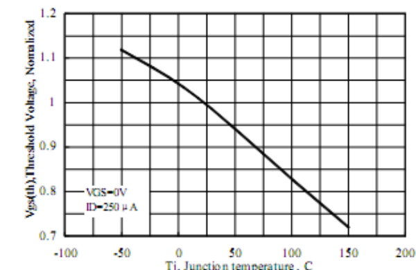
Figure 11 Typical Threshold Voltage vs Junction Temperature
