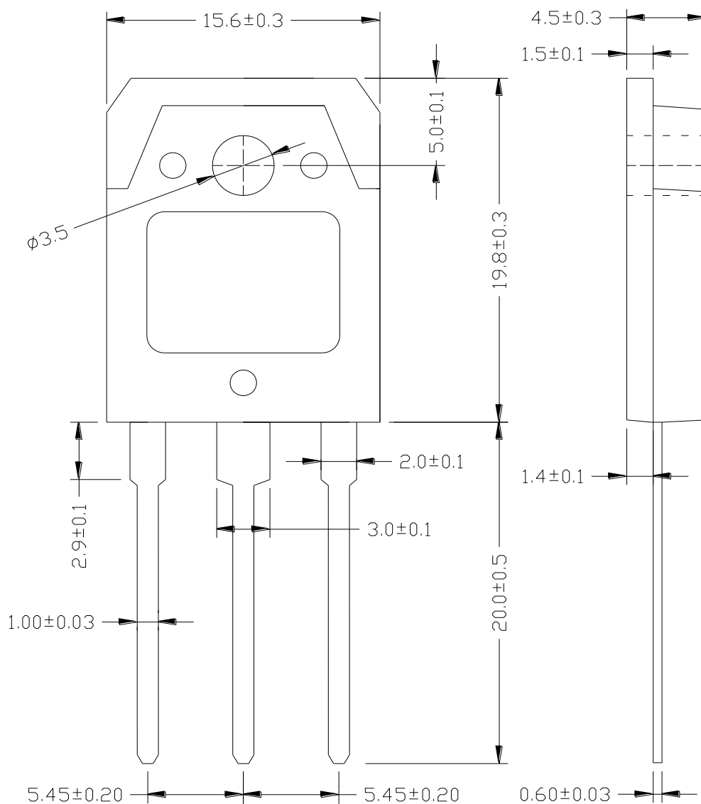
T0-3PB
