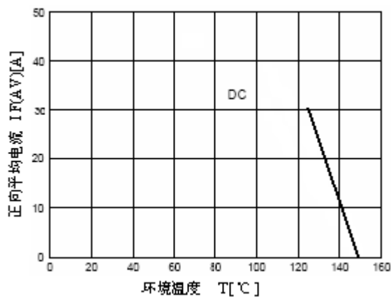
图 5. Forward Current Derating Curve
