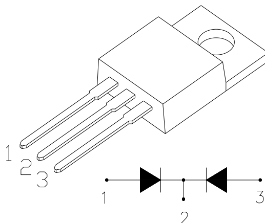
1. 阳极(A1) 2. 阴极(K) 3. 阳极(A2)
