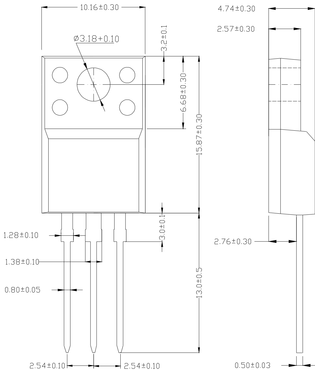
TO-220FH
